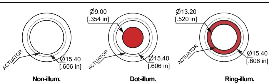
LENS OPTIONS
