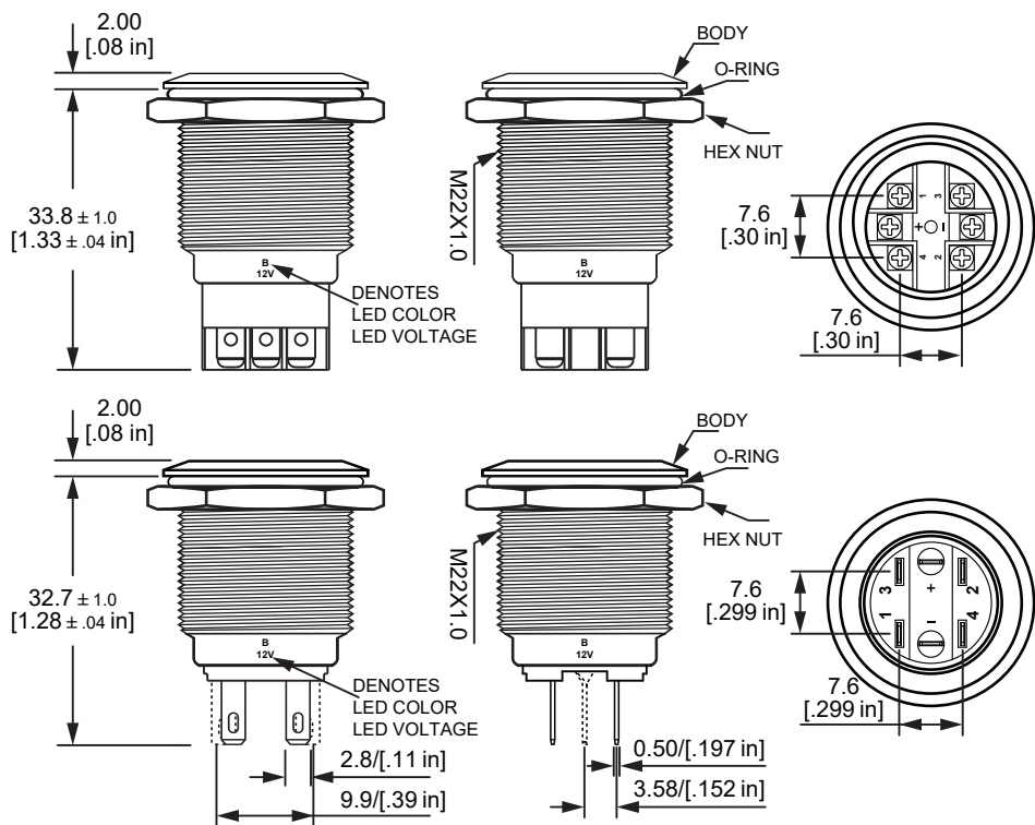
CONTACT CONFIGURATION ILLUMINATED
