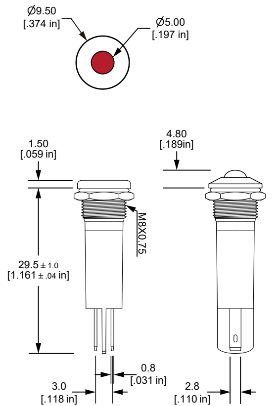
FLAT
