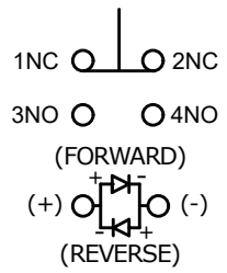
CONTACT CONFIGURATION ILLUMINATED
