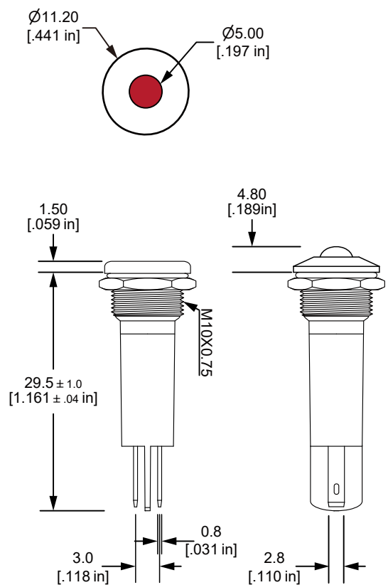
FLAT
