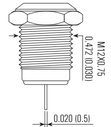
Momentary
